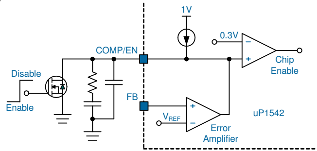
Figure 1. Chip Enable Function
